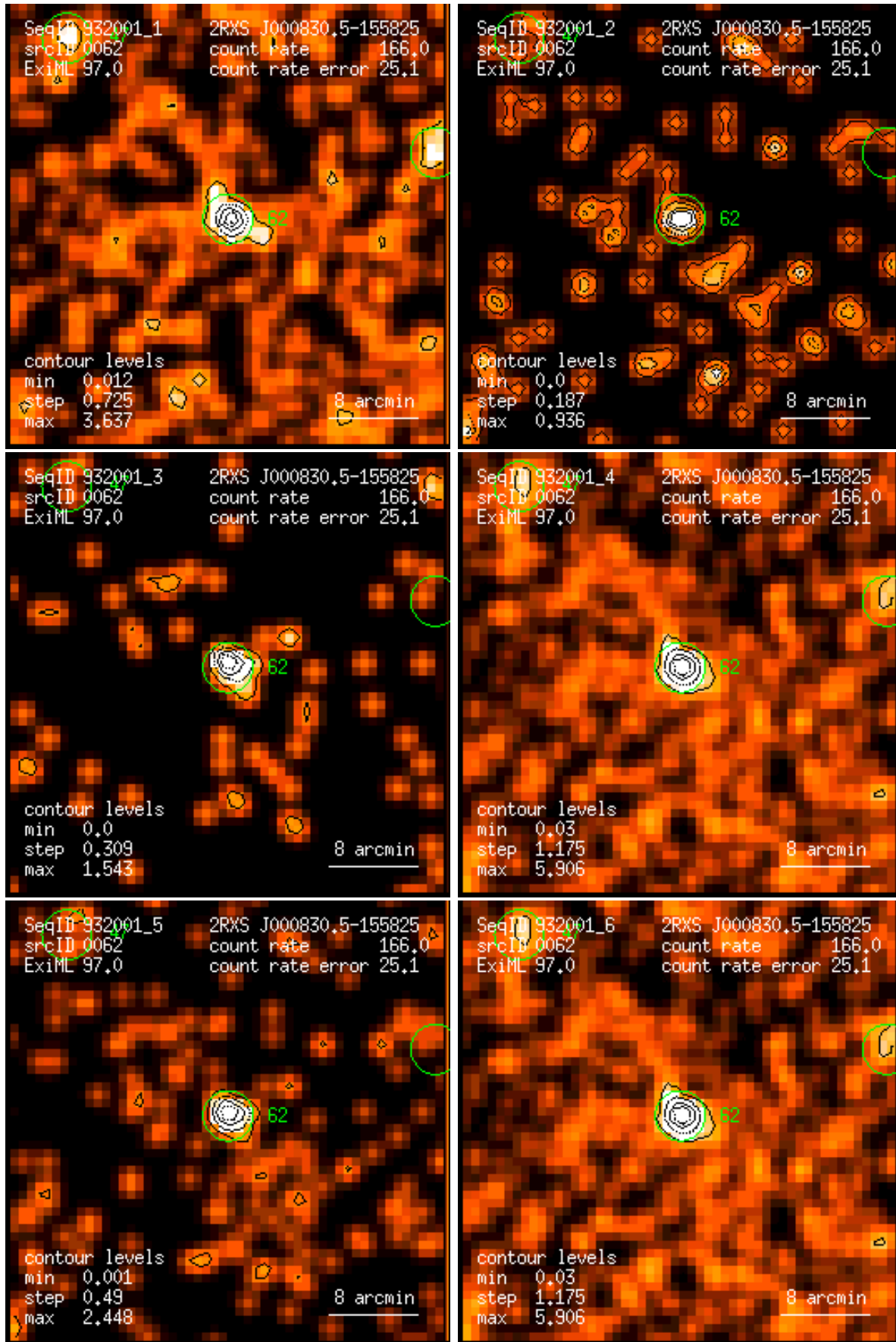
Figure 62: RASS 932001: detection 0062: band rate images, Gaussian filter: (1) PSPC channels 11 – 41, (2) 52 – 90, (3) 91 – 201, (4) 11 – 235, (5) 52 – 201, (6) 11 – 201. Broad band rates in counts/ks. Band rate contour levels in counts/ks/arcmin 2 .
