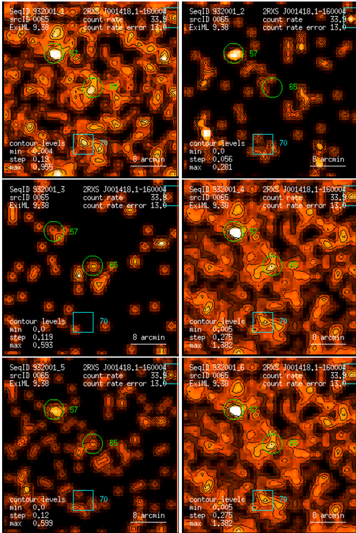
Figure 65: RASS 932001: detection 0065: band rate images, Gaussian filter: (1) PSPC channels 11 – 41, (2) 52 – 90, (3) 91 – 201, (4) 11 – 235, (5) 52 – 201, (6) 11 – 201. Broad band rates in counts/ks. Band rate contour levels in counts/ks/arcmin 2 .
