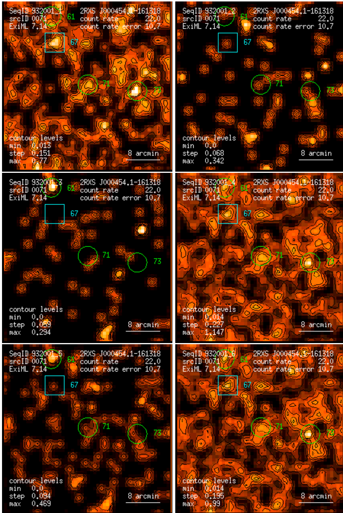
Figure 71: RASS 932001: detection 0071: band rate images, Gaussian filter: (1) PSPC channels 11 – 41, (2) 52 – 90, (3) 91 – 201, (4) 11 – 235, (5) 52 – 201, (6) 11 – 201. Broad band rates in counts/ks. Band rate contour levels in counts/ks/arcmin 2 .
