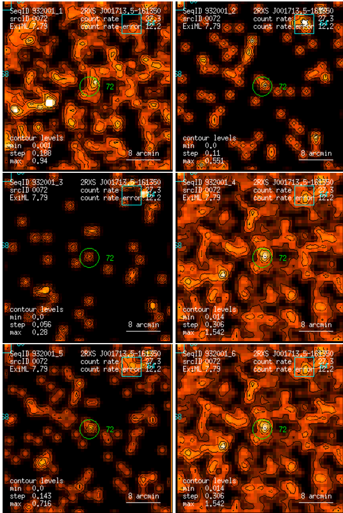
Figure 72: RASS 932001: detection 0072: band rate images, Gaussian filter: (1) PSPC channels 11 – 41, (2) 52 – 90, (3) 91 – 201, (4) 11 – 235, (5) 52 – 201, (6) 11 – 201. Broad band rates in counts/ks. Band rate contour levels in counts/ks/arcmin 2 .
