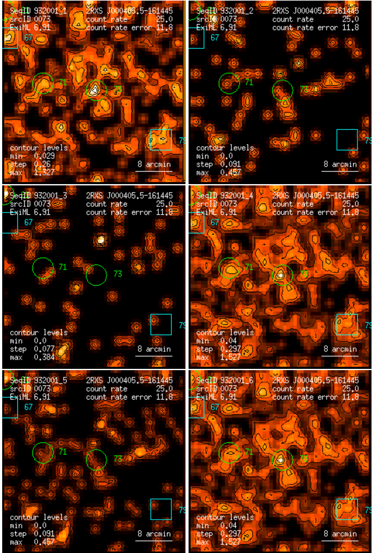
Figure 73: RASS 932001: detection 0073: band rate images, Gaussian filter: (1) PSPC channels 11 – 41, (2) 52 – 90, (3) 91 – 201, (4) 11 – 235, (5) 52 – 201, (6) 11 – 201. Broad band rates in counts/ks. Band rate contour levels in counts/ks/arcmin 2 .
