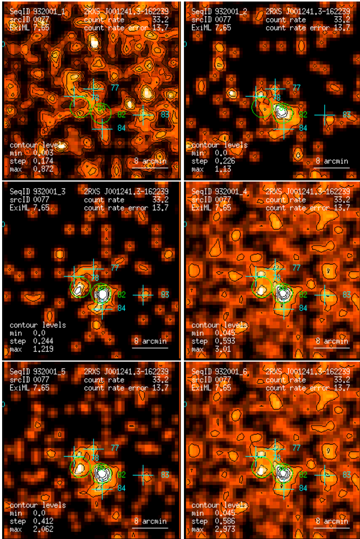
Figure 77: RASS 932001: detection 0077: band rate images, Gaussian filter: (1) PSPC channels 11 – 41, (2) 52 – 90, (3) 91 – 201, (4) 11 – 235, (5) 52 – 201, (6) 11 – 201. Broad band rates in counts/ks. Band rate contour levels in counts/ks/arcmin 2 .
