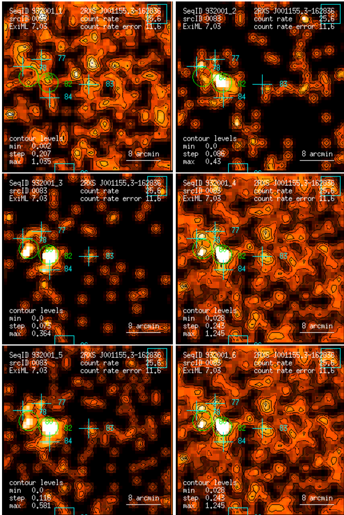
Figure 83: RASS 932001: detection 0083: band rate images, Gaussian filter: (1) PSPC channels 11 – 41, (2) 52 – 90, (3) 91 – 201, (4) 11 – 235, (5) 52 – 201, (6) 11 – 201. Broad band rates in counts/ks. Band rate contour levels in counts/ks/arcmin 2 .
