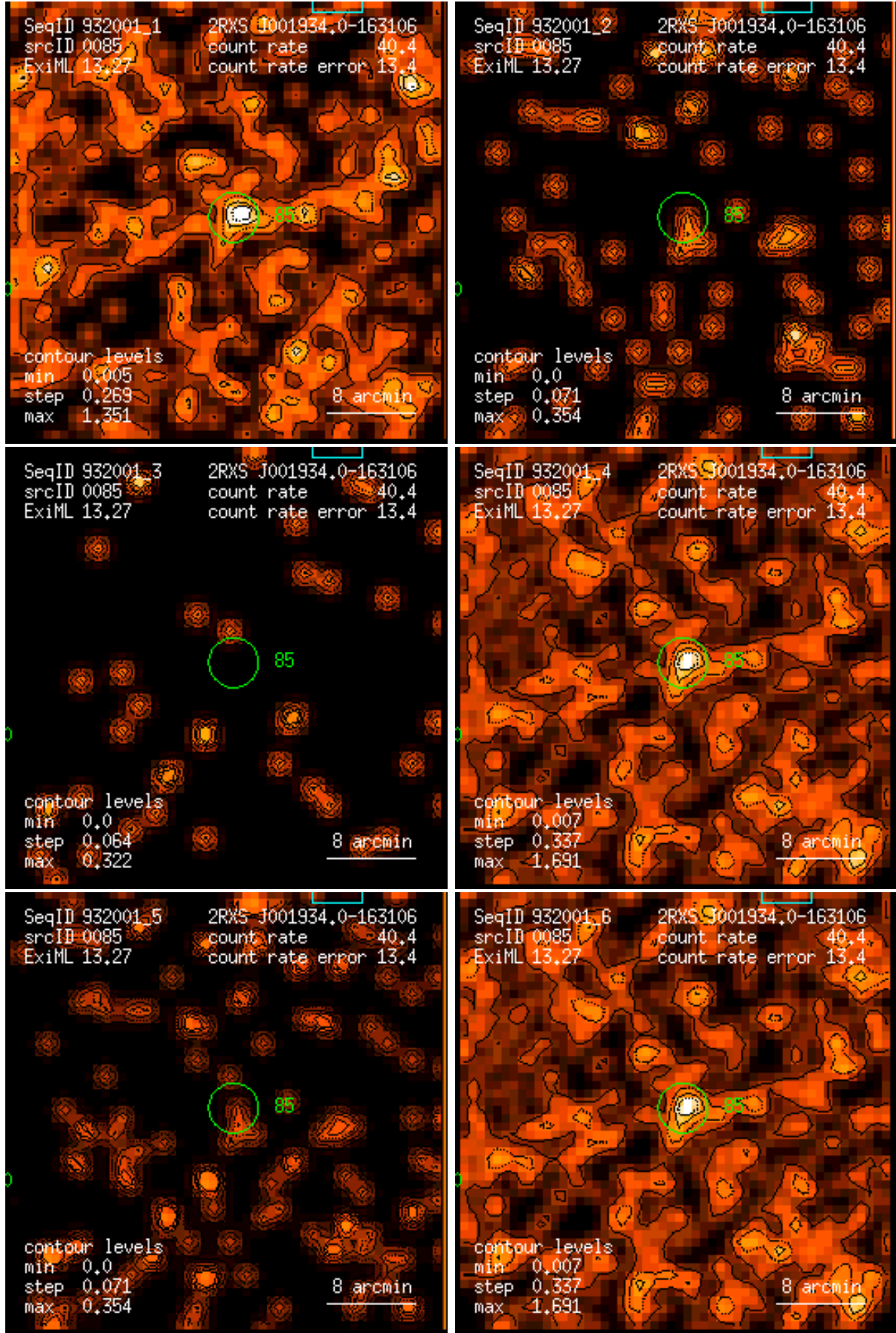
Figure 85: RASS 932001: detection 0085: band rate images, Gaussian filter: (1) PSPC channels 11 – 41, (2) 52 – 90, (3) 91 – 201, (4) 11 – 235, (5) 52 – 201, (6) 11 – 201. Broad band rates in counts/ks. Band rate contour levels in counts/ks/arcmin 2 .
