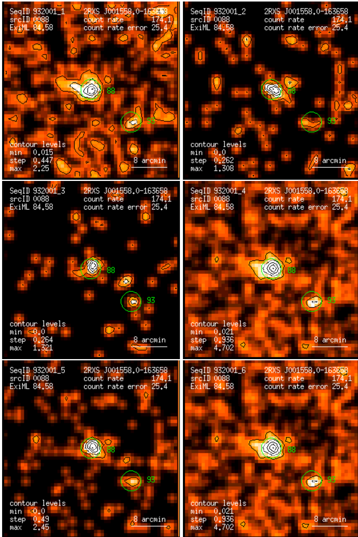
Figure 88: RASS 932001: detection 0088: band rate images, Gaussian filter: (1) PSPC channels 11 – 41, (2) 52 – 90, (3) 91 – 201, (4) 11 – 235, (5) 52 – 201, (6) 11 – 201. Broad band rates in counts/ks. Band rate contour levels in counts/ks/arcmin 2 .
