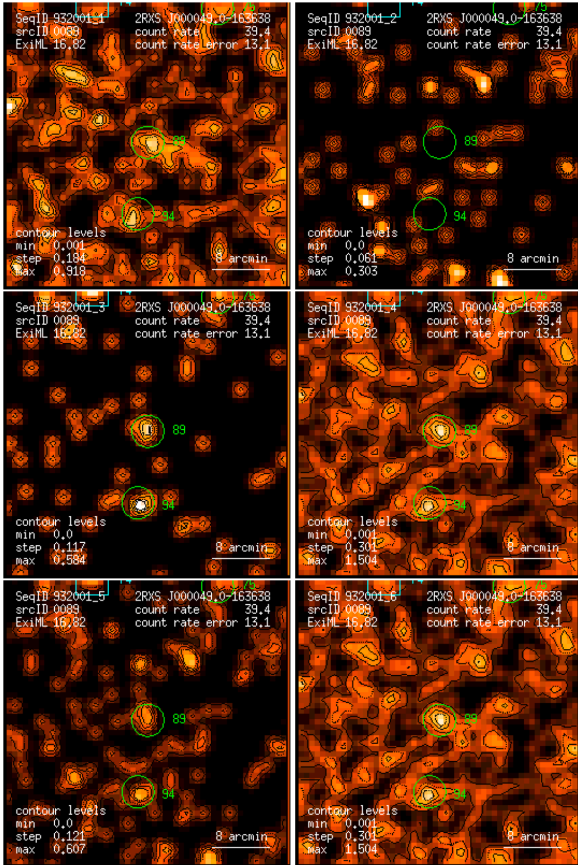
Figure 89: RASS 932001: detection 0089: band rate images, Gaussian filter: (1) PSPC channels 11 – 41, (2) 52 – 90, (3) 91 – 201, (4) 11 – 235, (5) 52 – 201, (6) 11 – 201. Broad band rates in counts/ks. Band rate contour levels in counts/ks/arcmin 2 .
