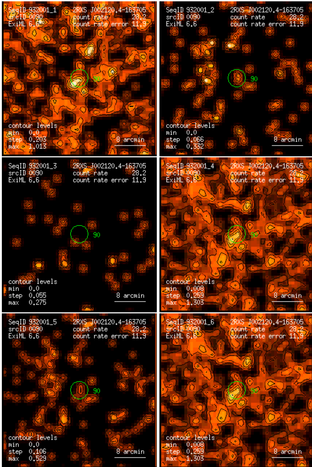
Figure 90: RASS 932001: detection 0090: band rate images, Gaussian filter: (1) PSPC channels 11 – 41, (2) 52 – 90, (3) 91 – 201, (4) 11 – 235, (5) 52 – 201, (6) 11 – 201. Broad band rates in counts/ks. Band rate contour levels in counts/ks/arcmin 2 .
