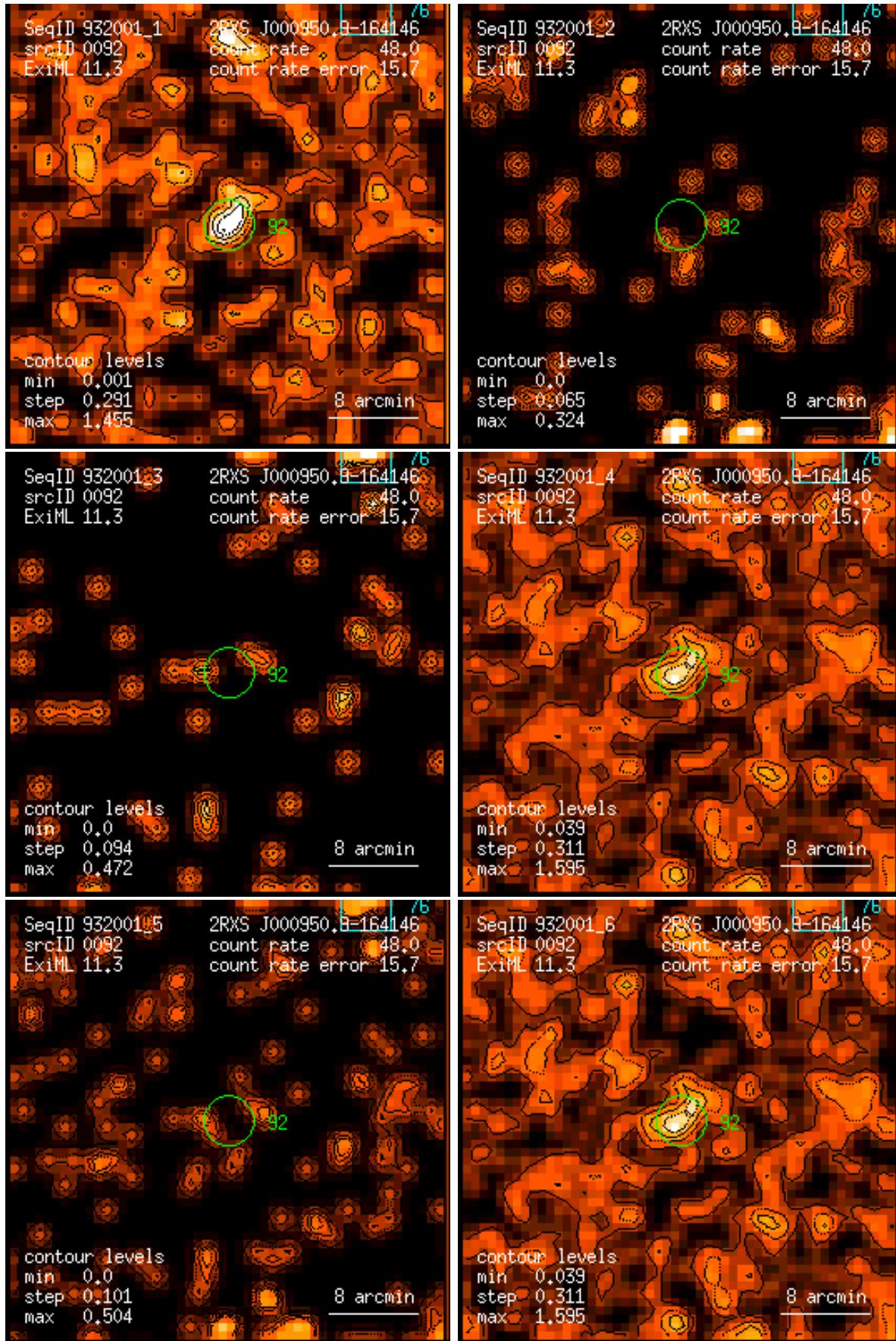
Figure 92: RASS 932001: detection 0092: band rate images, Gaussian filter: (1) PSPC channels 11 – 41, (2) 52 – 90, (3) 91 – 201, (4) 11 – 235, (5) 52 – 201, (6) 11 – 201. Broad band rates in counts/ks. Band rate contour levels in counts/ks/arcmin 2 .
