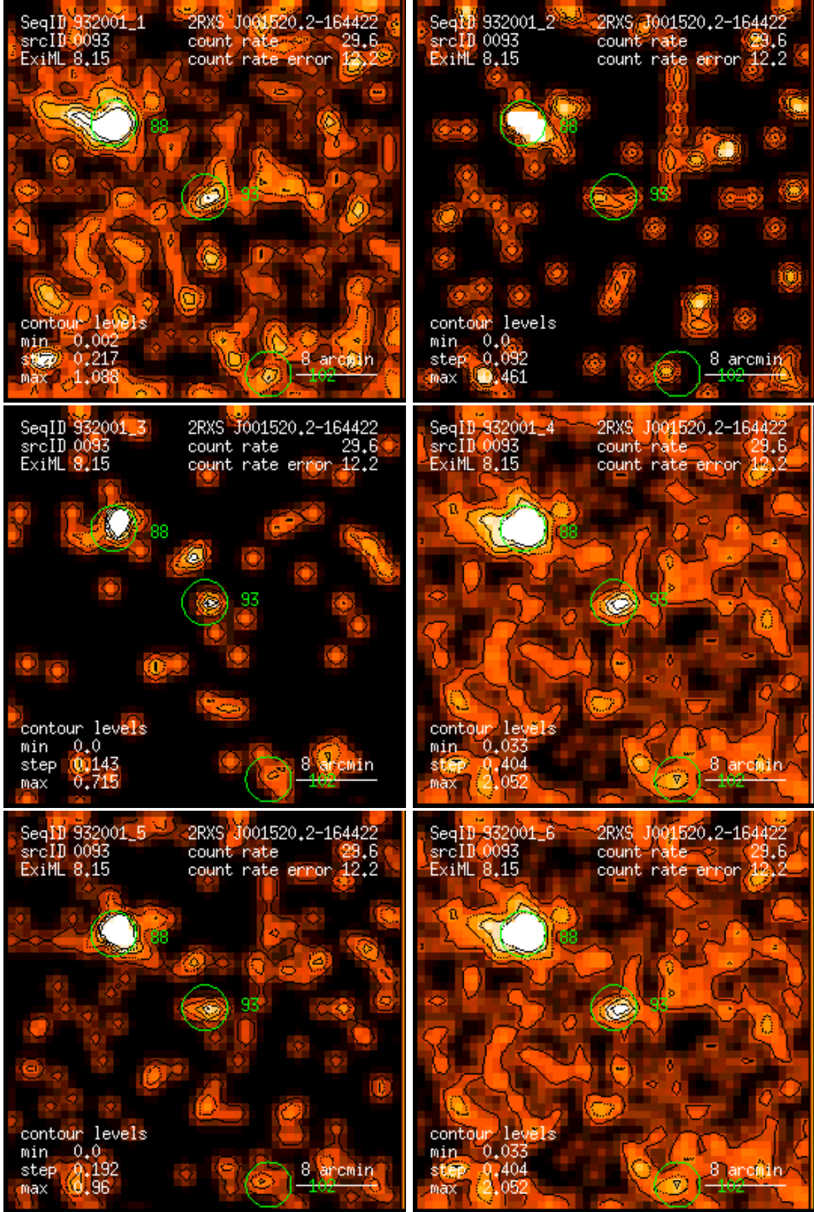
Figure 93: RASS 932001: detection 0093: band rate images, Gaussian filter: (1) PSPC channels 11 – 41, (2) 52 – 90, (3) 91 – 201, (4) 11 – 235, (5) 52 – 201, (6) 11 – 201. Broad band rates in counts/ks. Band rate contour levels in counts/ks/arcmin 2 .
