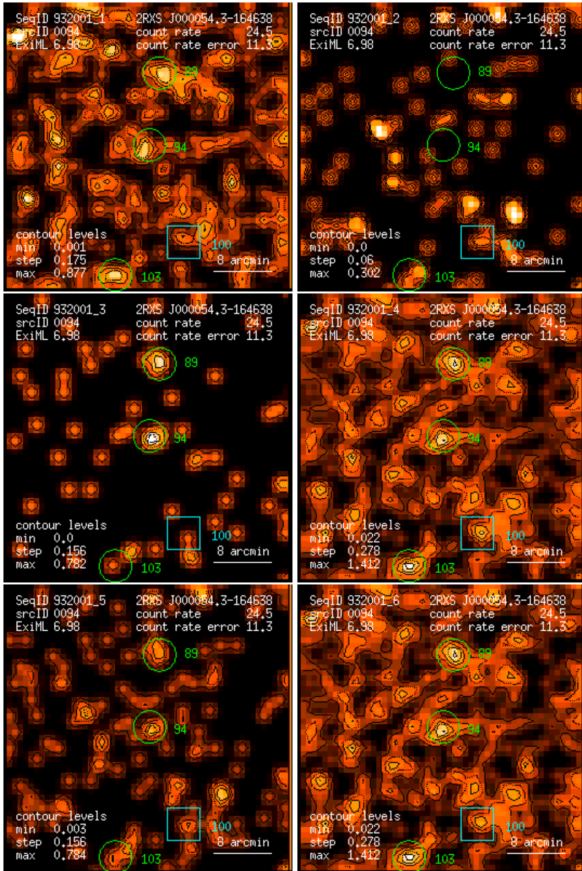
Figure 94: RASS 932001: detection 0094: band rate images, Gaussian filter: (1) PSPC channels 11 – 41, (2) 52 – 90, (3) 91 – 201, (4) 11 – 235, (5) 52 – 201, (6) 11 – 201. Broad band rates in counts/ks. Band rate contour levels in counts/ks/arcmin 2 .
