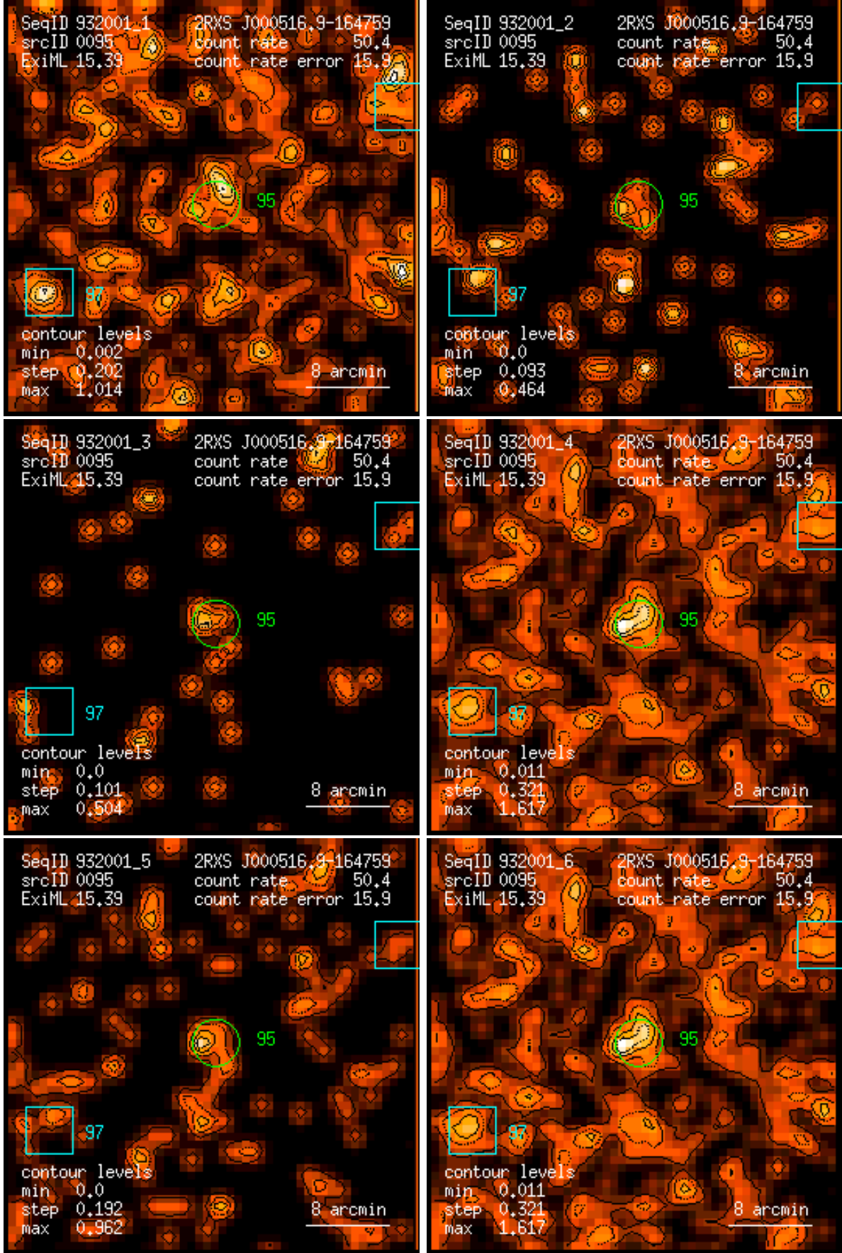
Figure 95: RASS 932001: detection 0095: band rate images, Gaussian filter: (1) PSPC channels 11 – 41, (2) 52 – 90, (3) 91 – 201, (4) 11 – 235, (5) 52 – 201, (6) 11 – 201. Broad band rates in counts/ks. Band rate contour levels in counts/ks/arcmin 2 .
