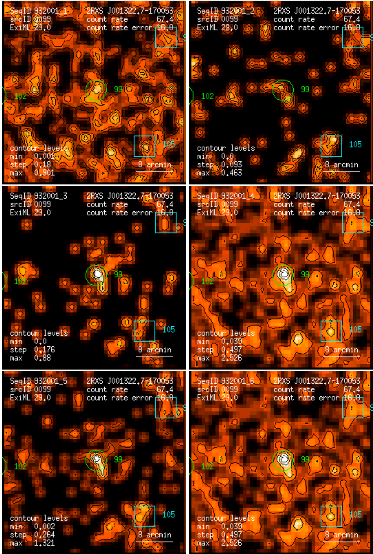
Figure 99: RASS 932001: detection 0099: band rate images, Gaussian filter: (1) PSPC channels 11 – 41, (2) 52 – 90, (3) 91 – 201, (4) 11 – 235, (5) 52 – 201, (6) 11 – 201. Broad band rates in counts/ks. Band rate contour levels in counts/ks/arcmin 2 .
