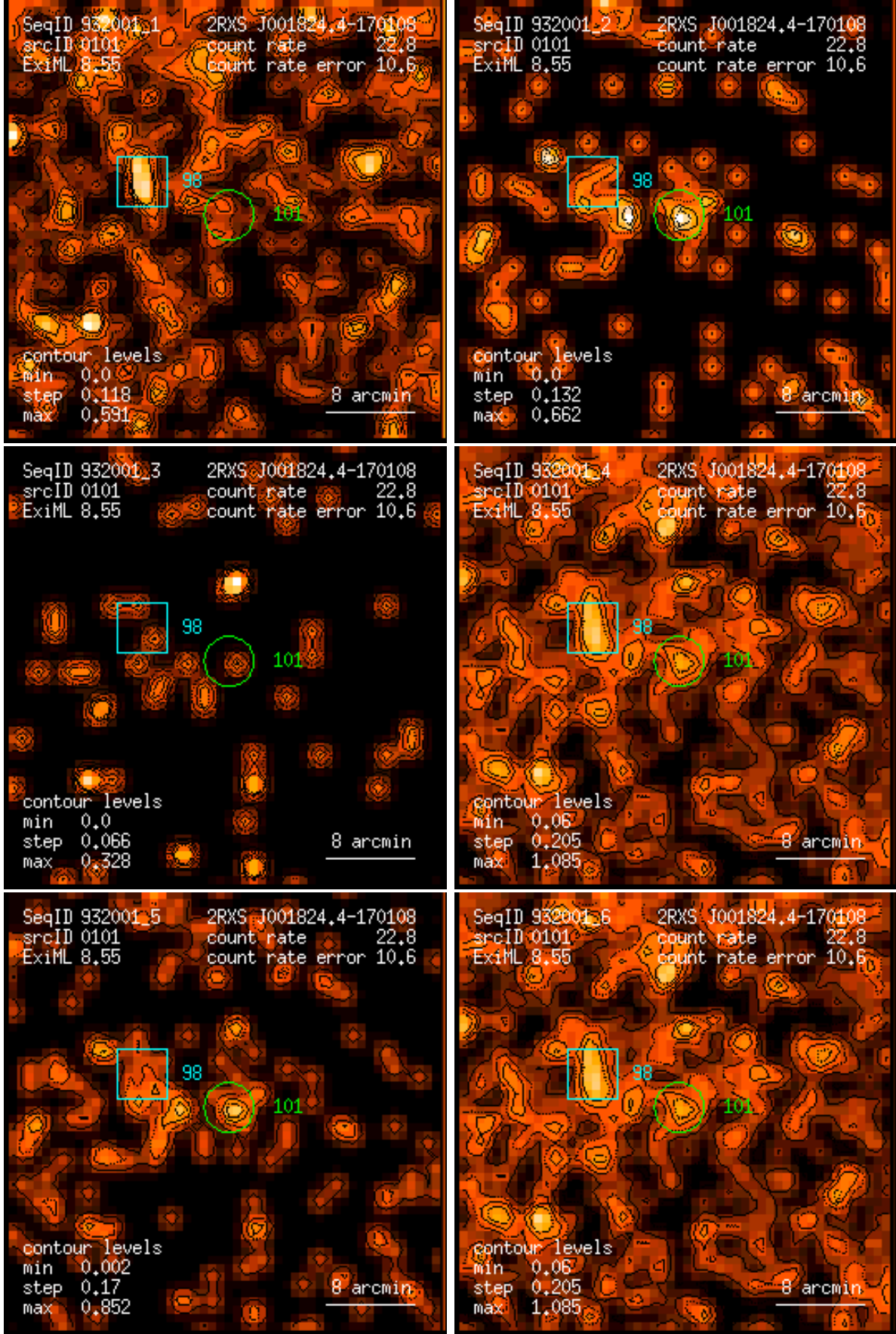
Figure 101: RASS 932001: detection 0101: band rate images, Gaussian filter: (1) PSPC channels 11 – 41, (2) 52 – 90, (3) 91 – 201, (4) 11 – 235, (5) 52 – 201, (6) 11 – 201. Broad band rates in counts/ks. Band rate contour levels in counts/ks/arcmin 2 .
