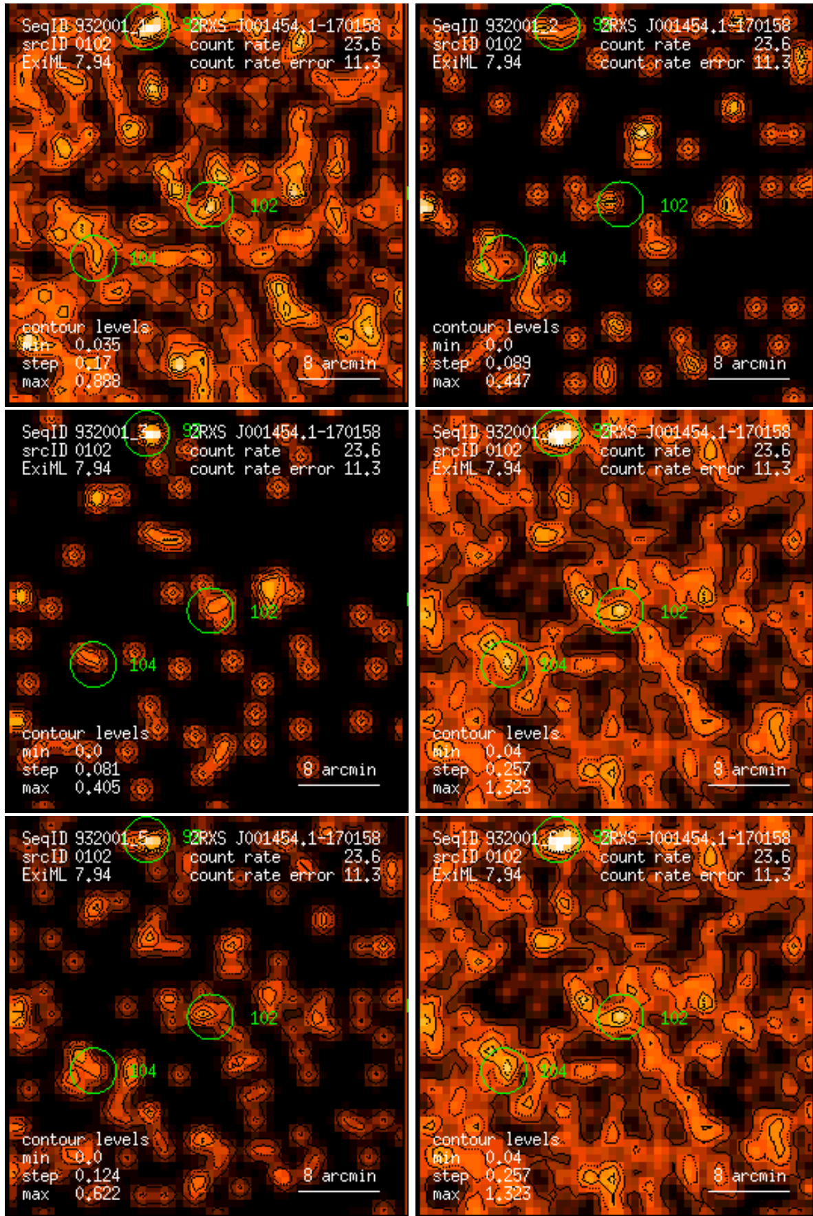
Figure 102: RASS 932001: detection 0102: band rate images, Gaussian filter: (1) PSPC channels 11 – 41, (2) 52 – 90, (3) 91 – 201, (4) 11 – 235, (5) 52 – 201, (6) 11 – 201. Broad band rates in counts/ks. Band rate contour levels in counts/ks/arcmin 2 .
