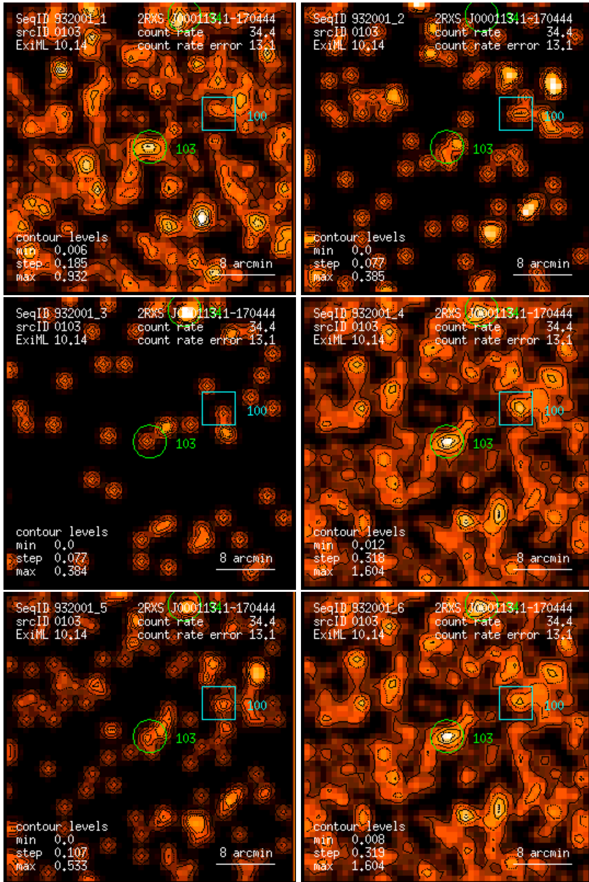
Figure 103: RASS 932001: detection 0103: band rate images, Gaussian filter: (1) PSPC channels 11 – 41, (2) 52 – 90, (3) 91 – 201, (4) 11 – 235, (5) 52 – 201, (6) 11 – 201. Broad band rates in counts/ks. Band rate contour levels in counts/ks/arcmin 2 .
