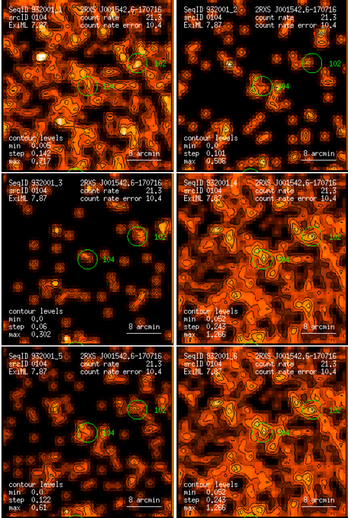
Figure 104: RASS 932001: detection 0104: band rate images, Gaussian filter: (1) PSPC channels 11 – 41, (2) 52 – 90, (3) 91 – 201, (4) 11 – 235, (5) 52 – 201, (6) 11 – 201. Broad band rates in counts/ks. Band rate contour levels in counts/ks/arcmin 2 .
