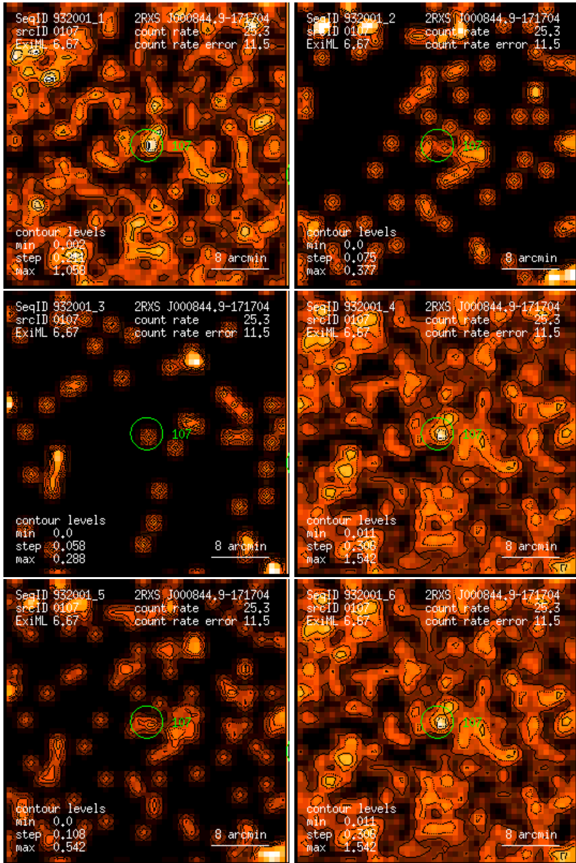
Figure 107: RASS 932001: detection 0107: band rate images, Gaussian filter: (1) PSPC channels 11 – 41, (2) 52 – 90, (3) 91 – 201, (4) 11 – 235, (5) 52 – 201, (6) 11 – 201. Broad band rates in counts/ks. Band rate contour levels in counts/ks/arcmin 2 .
