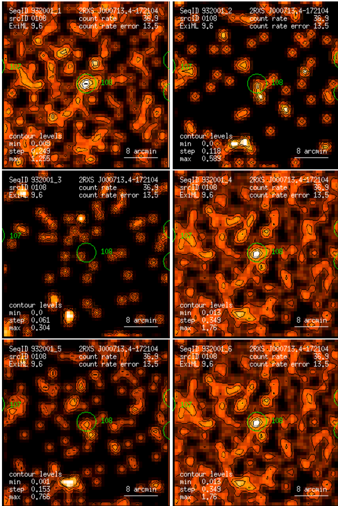
Figure 108: RASS 932001: detection 0108: band rate images, Gaussian filter: (1) PSPC channels 11 – 41, (2) 52 – 90, (3) 91 – 201, (4) 11 – 235, (5) 52 – 201, (6) 11 – 201. Broad band rates in counts/ks. Band rate contour levels in counts/ks/arcmin 2 .
