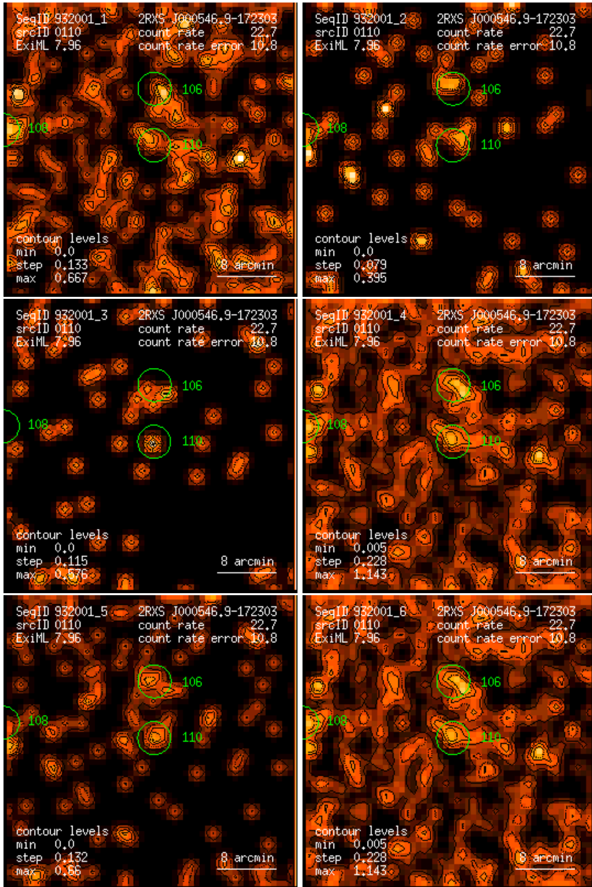
Figure 110: RASS 932001: detection 0110: band rate images, Gaussian filter: (1) PSPC channels 11 – 41, (2) 52 – 90, (3) 91 – 201, (4) 11 – 235, (5) 52 – 201, (6) 11 – 201. Broad band rates in counts/ks. Band rate contour levels in counts/ks/arcmin 2 .
