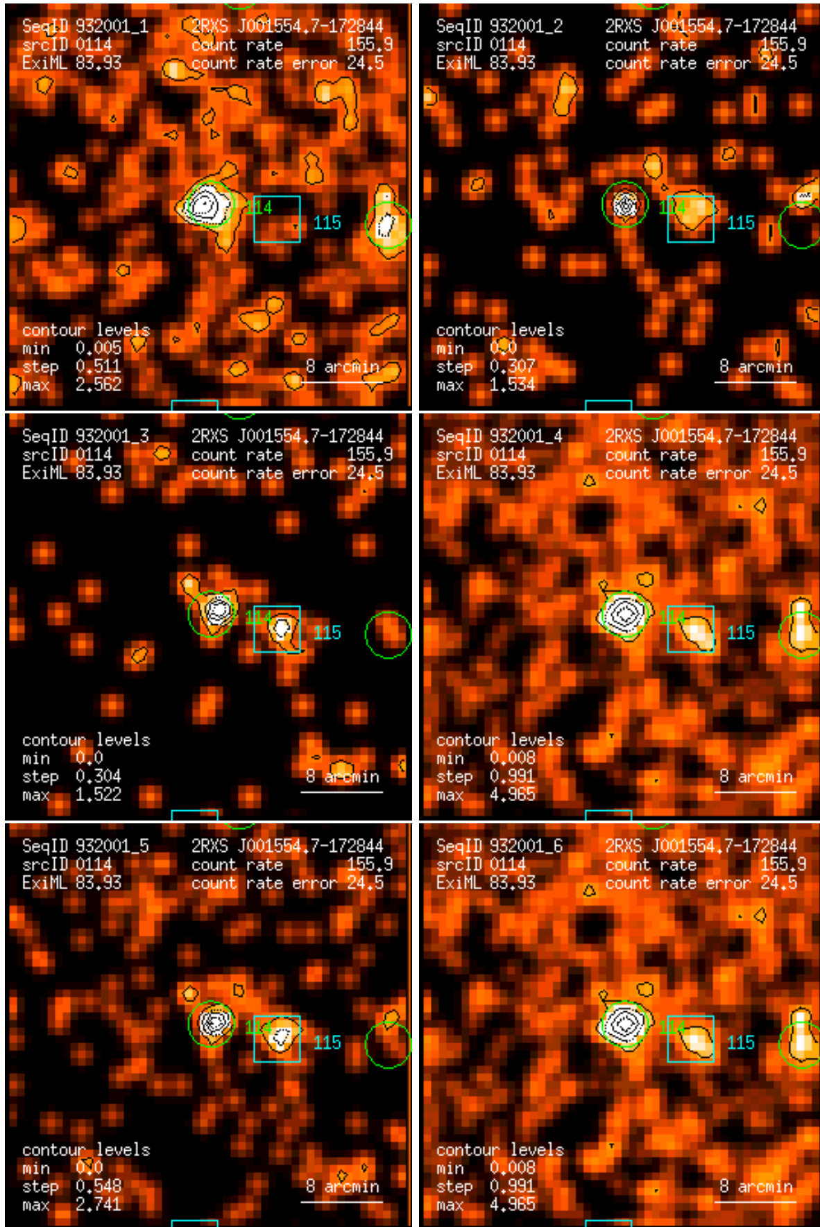
Figure 114: RASS 932001: detection 0114: band rate images, Gaussian filter: (1) PSPC channels 11 – 41, (2) 52 – 90, (3) 91 – 201, (4) 11 – 235, (5) 52 – 201, (6) 11 – 201. Broad band rates in counts/ks. Band rate contour levels in counts/ks/arcmin 2 .
