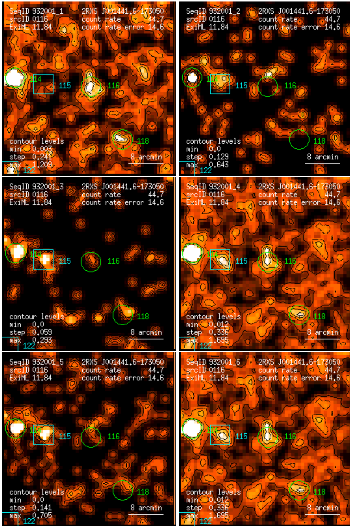
Figure 116: RASS 932001: detection 0116: band rate images, Gaussian filter: (1) PSPC channels 11 – 41, (2) 52 – 90, (3) 91 – 201, (4) 11 – 235, (5) 52 – 201, (6) 11 – 201. Broad band rates in counts/ks. Band rate contour levels in counts/ks/arcmin 2 .
