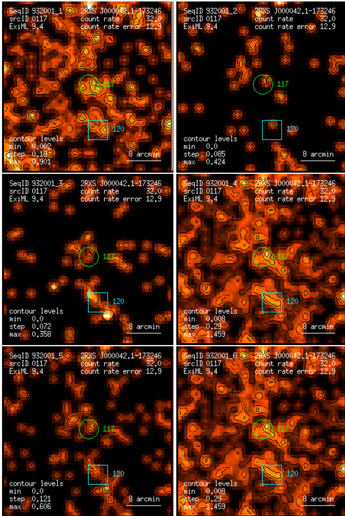
Figure 117: RASS 932001: detection 0117: band rate images, Gaussian filter: (1) PSPC channels 11 – 41, (2) 52 – 90, (3) 91 – 201, (4) 11 – 235, (5) 52 – 201, (6) 11 – 201. Broad band rates in counts/ks. Band rate contour levels in counts/ks/arcmin 2 .
