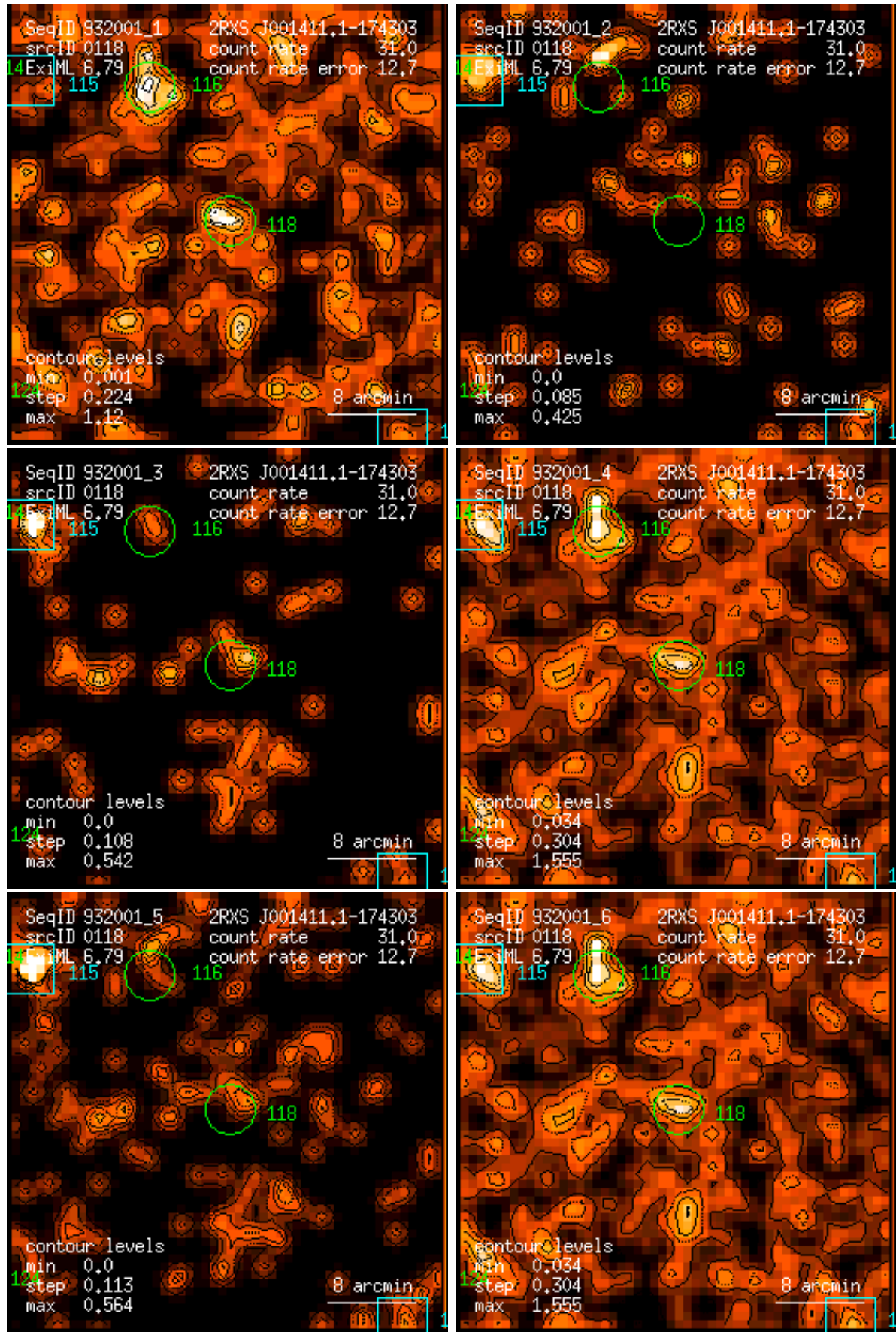
Figure 118: RASS 932001: detection 0118: band rate images, Gaussian filter: (1) PSPC channels 11 – 41, (2) 52 – 90, (3) 91 – 201, (4) 11 – 235, (5) 52 – 201, (6) 11 – 201. Broad band rates in counts/ks. Band rate contour levels in counts/ks/arcmin 2 .
