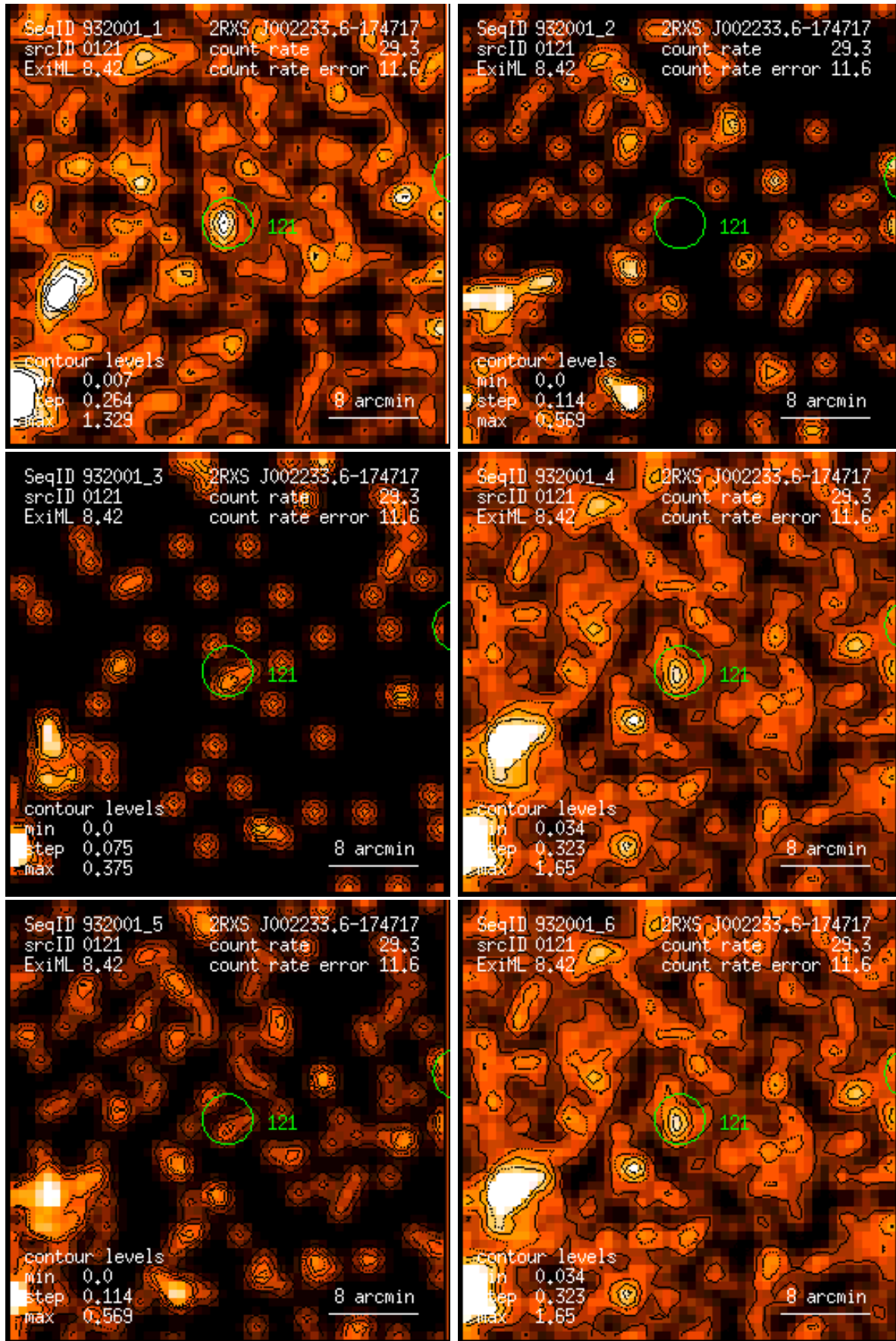
Figure 121: RASS 932001: detection 0121: band rate images, Gaussian filter: (1) PSPC channels 11 – 41, (2) 52 – 90, (3) 91 – 201, (4) 11 – 235, (5) 52 – 201, (6) 11 – 201. Broad band rates in counts/ks. Band rate contour levels in counts/ks/arcmin 2 .
