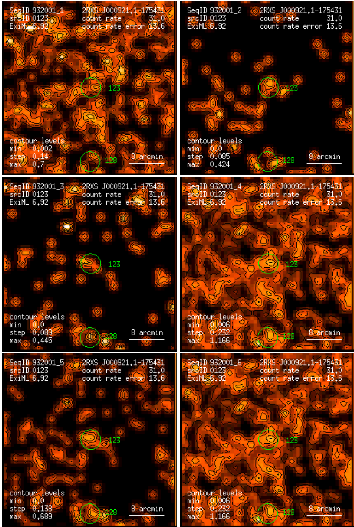
Figure 123: RASS 932001: detection 0123: band rate images, Gaussian filter: (1) PSPC channels 11 – 41, (2) 52 – 90, (3) 91 – 201, (4) 11 – 235, (5) 52 – 201, (6) 11 – 201. Broad band rates in counts/ks. Band rate contour levels in counts/ks/arcmin 2 .
