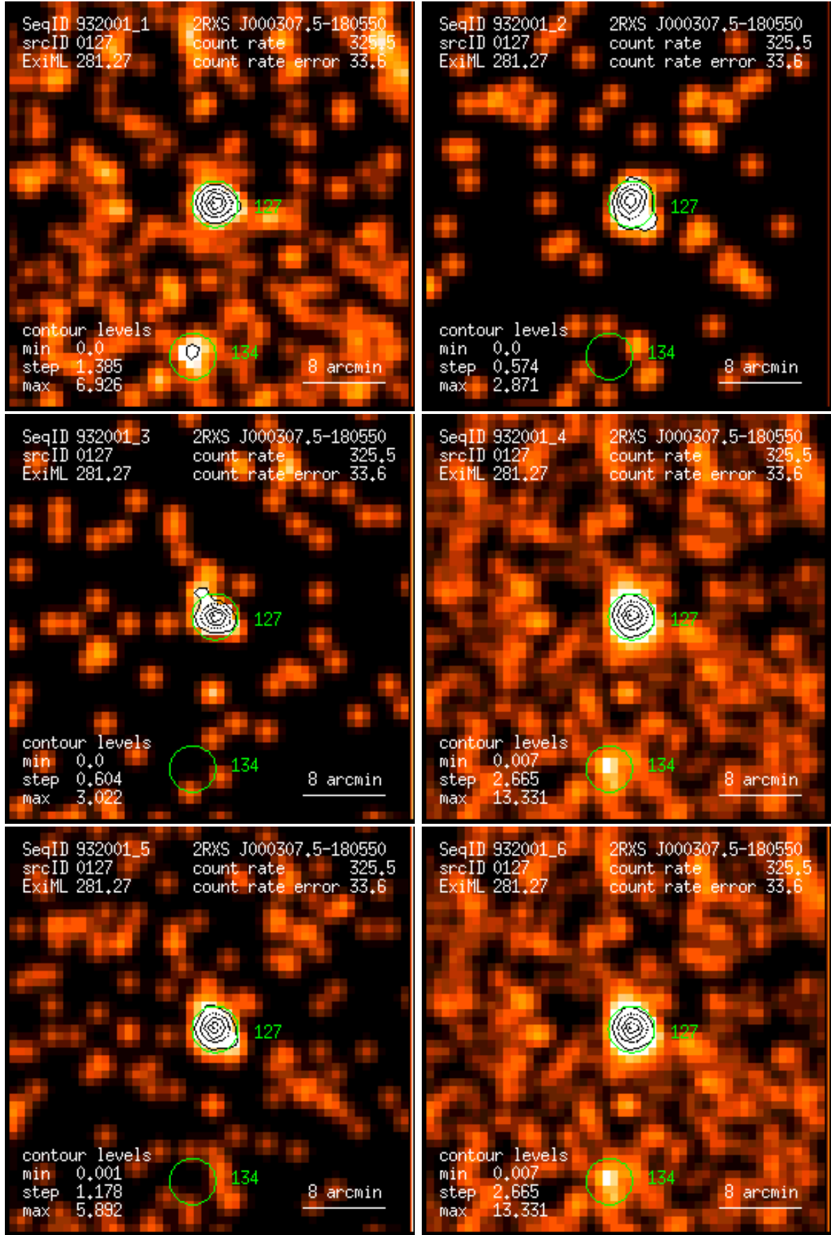
Figure 127: RASS 932001: detection 0127: band rate images, Gaussian filter: (1) PSPC channels 11 – 41, (2) 52 – 90, (3) 91 – 201, (4) 11 – 235, (5) 52 – 201, (6) 11 – 201. Broad band rates in counts/ks. Band rate contour levels in counts/ks/arcmin 2 .
