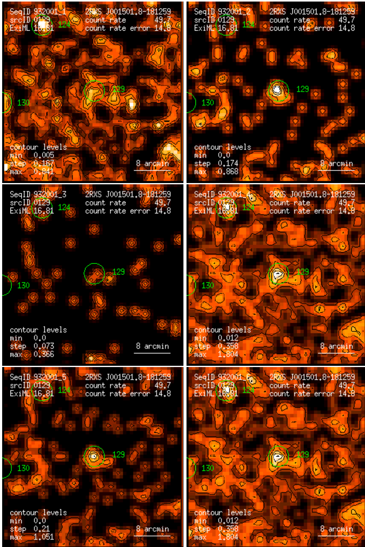
Figure 129: RASS 932001: detection 0129: band rate images, Gaussian filter: (1) PSPC channels 11 – 41, (2) 52 – 90, (3) 91 – 201, (4) 11 – 235, (5) 52 – 201, (6) 11 – 201. Broad band rates in counts/ks. Band rate contour levels in counts/ks/arcmin 2 .
