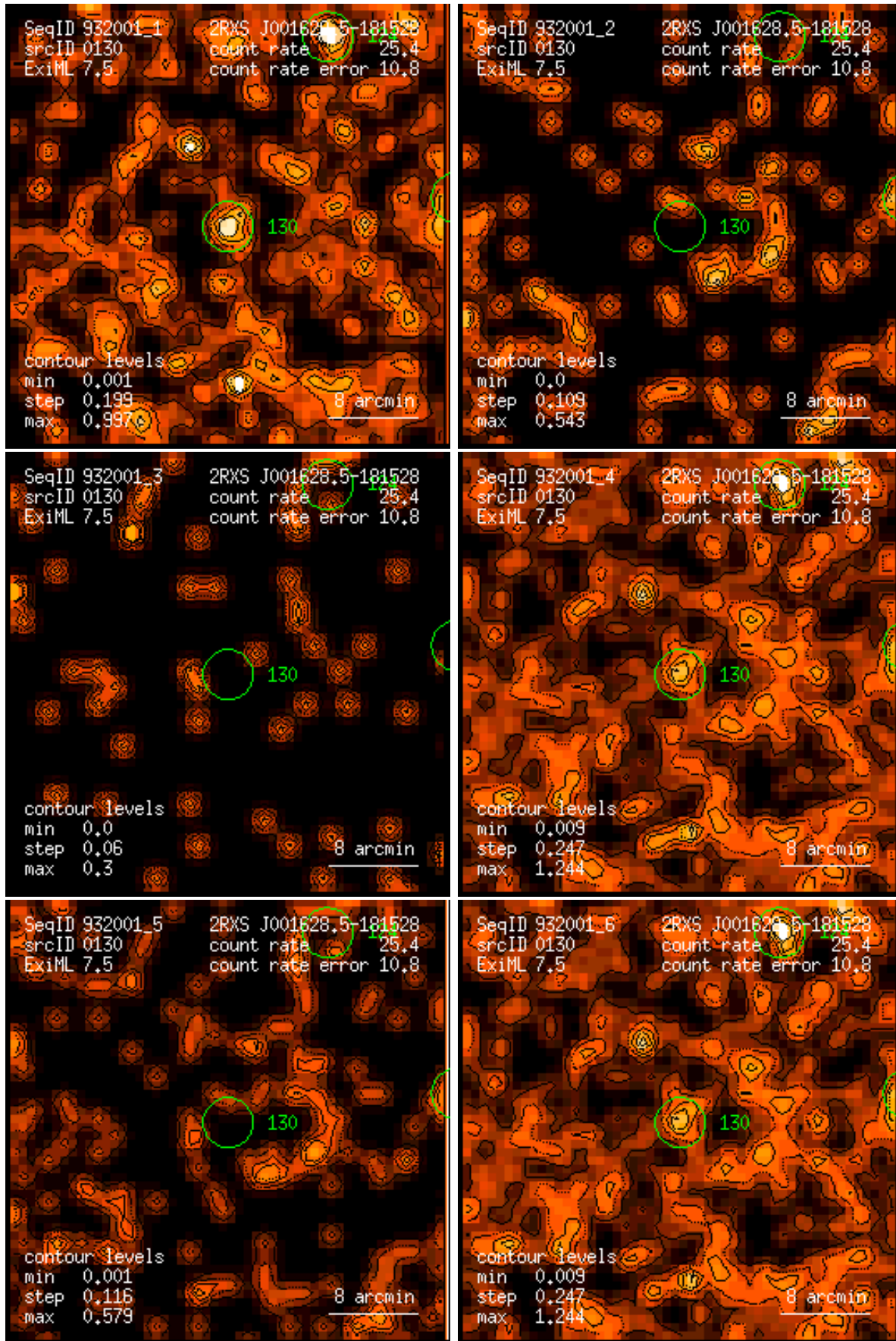
Figure 130: RASS 932001: detection 0130: band rate images, Gaussian filter: (1) PSPC channels 11 – 41, (2) 52 – 90, (3) 91 – 201, (4) 11 – 235, (5) 52 – 201, (6) 11 – 201. Broad band rates in counts/ks. Band rate contour levels in counts/ks/arcmin 2 .
