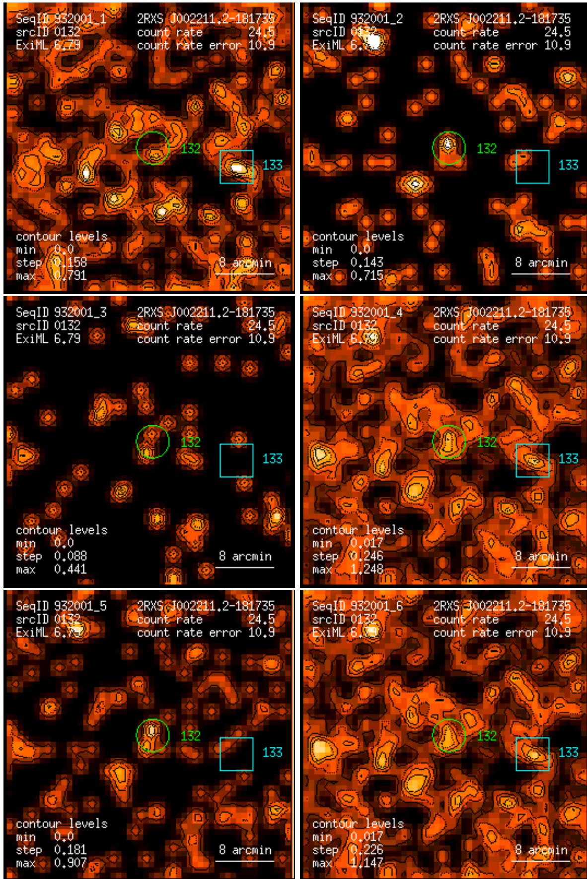
Figure 132: RASS 932001: detection 0132: band rate images, Gaussian filter: (1) PSPC channels 11 – 41, (2) 52 – 90, (3) 91 – 201, (4) 11 – 235, (5) 52 – 201, (6) 11 – 201. Broad band rates in counts/ks. Band rate contour levels in counts/ks/arcmin 2 .
