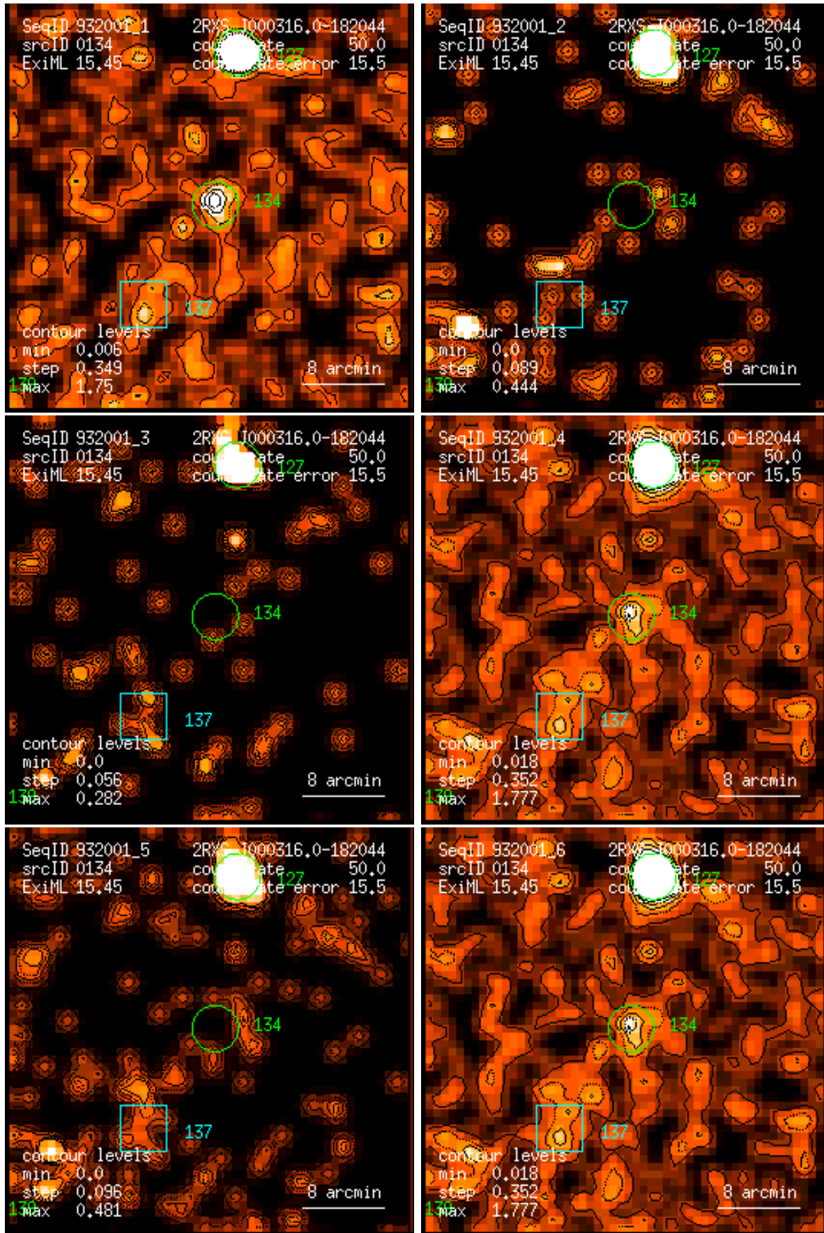
Figure 134: RASS 932001: detection 0134: band rate images, Gaussian filter: (1) PSPC channels 11 – 41, (2) 52 – 90, (3) 91 – 201, (4) 11 – 235, (5) 52 – 201, (6) 11 – 201. Broad band rates in counts/ks. Band rate contour levels in counts/ks/arcmin 2 .
