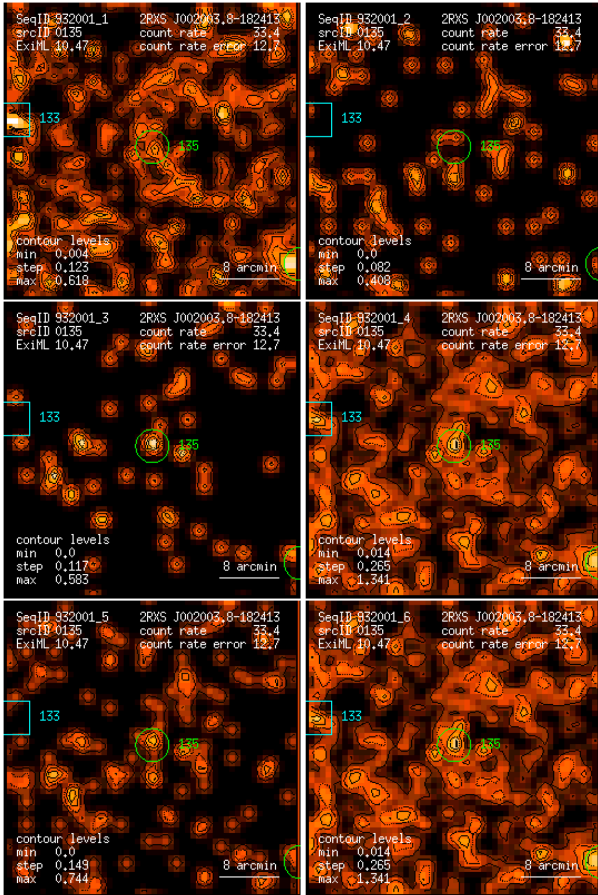
Figure 135: RASS 932001: detection 0135: band rate images, Gaussian filter: (1) PSPC channels 11 – 41, (2) 52 – 90, (3) 91 – 201, (4) 11 – 235, (5) 52 – 201, (6) 11 – 201. Broad band rates in counts/ks. Band rate contour levels in counts/ks/arcmin 2 .
