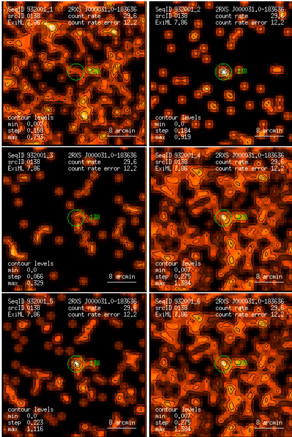
Figure 138: RASS 932001: detection 0138: band rate images, Gaussian filter: (1) PSPC channels 11 – 41, (2) 52 – 90, (3) 91 – 201, (4) 11 – 235, (5) 52 – 201, (6) 11 – 201. Broad band rates in counts/ks. Band rate contour levels in counts/ks/arcmin 2 .
