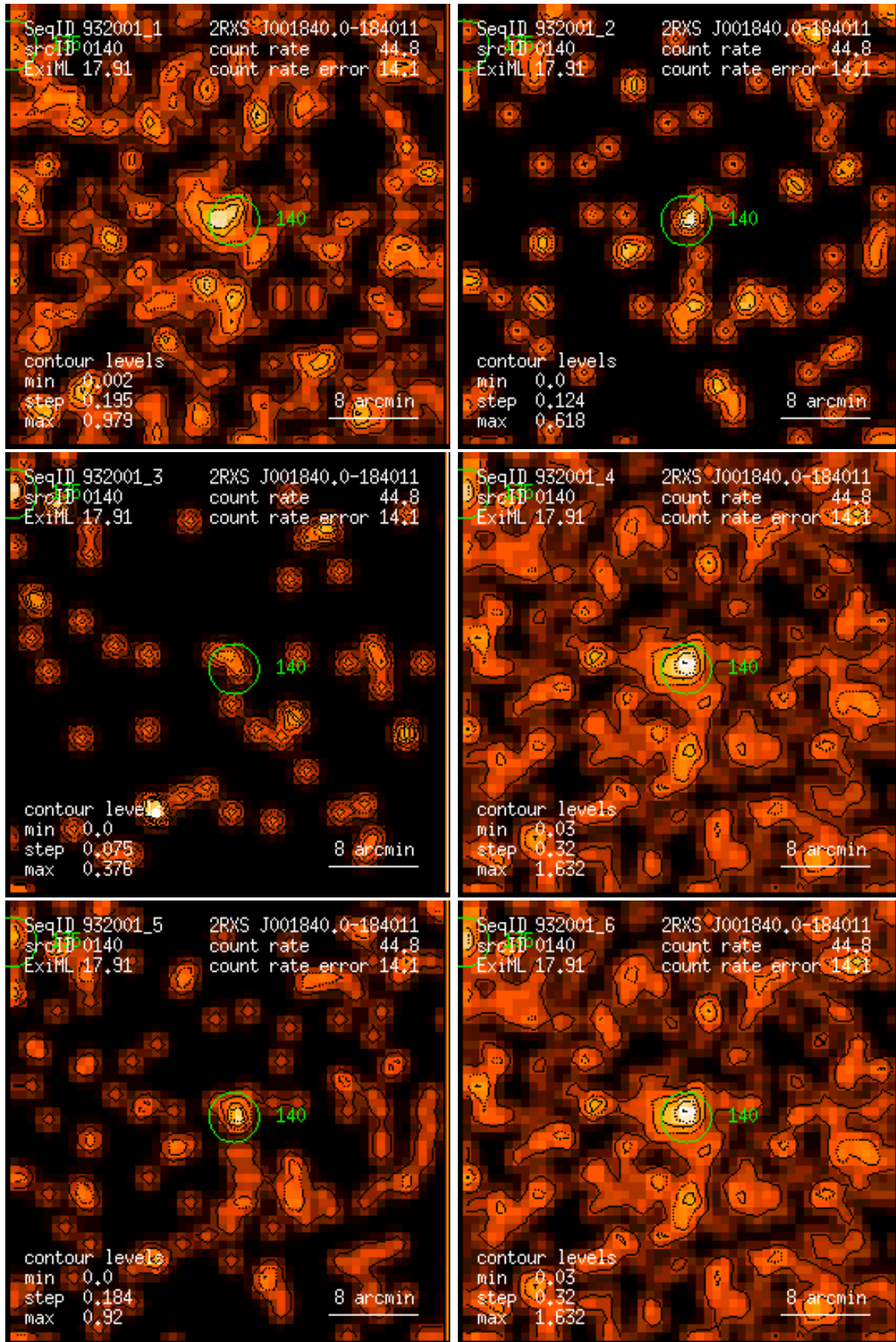
Figure 140: RASS 932001: detection 0140: band rate images, Gaussian filter: (1) PSPC channels 11 – 41, (2) 52 – 90, (3) 91 – 201, (4) 11 – 235, (5) 52 – 201, (6) 11 – 201. Broad band rates in counts/ks. Band rate contour levels in counts/ks/arcmin 2 .
