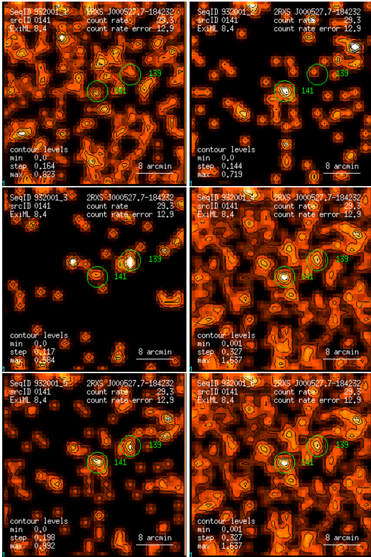
Figure 141: RASS 932001: detection 0141: band rate images, Gaussian filter: (1) PSPC channels 11 – 41, (2) 52 – 90, (3) 91 – 201, (4) 11 – 235, (5) 52 – 201, (6) 11 – 201. Broad band rates in counts/ks. Band rate contour levels in counts/ks/arcmin 2 .
