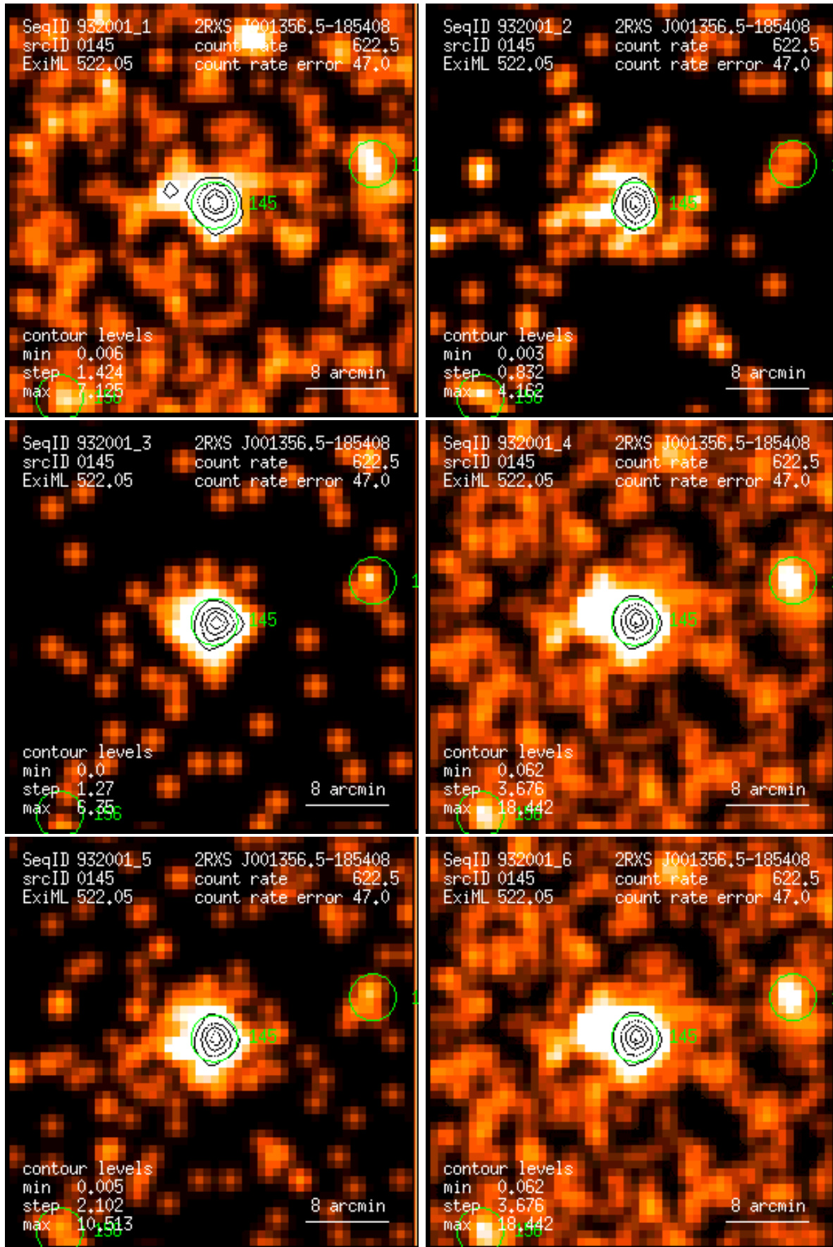
Figure 145: RASS 932001: detection 0145: band rate images, Gaussian filter: (1) PSPC channels 11 – 41, (2) 52 – 90, (3) 91 – 201, (4) 11 – 235, (5) 52 – 201, (6) 11 – 201. Broad band rates in counts/ks. Band rate contour levels in counts/ks/arcmin 2 .
