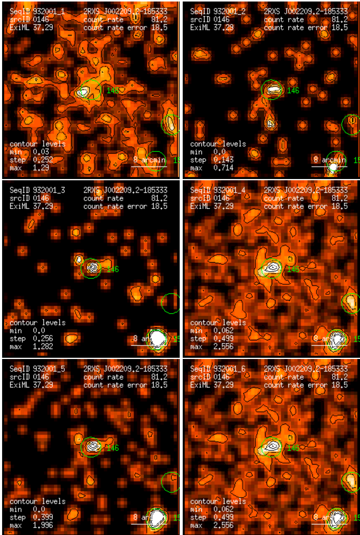
Figure 146: RASS 932001: detection 0146: band rate images, Gaussian filter: (1) PSPC channels 11 – 41, (2) 52 – 90, (3) 91 – 201, (4) 11 – 235, (5) 52 – 201, (6) 11 – 201. Broad band rates in counts/ks. Band rate contour levels in counts/ks/arcmin 2 .
