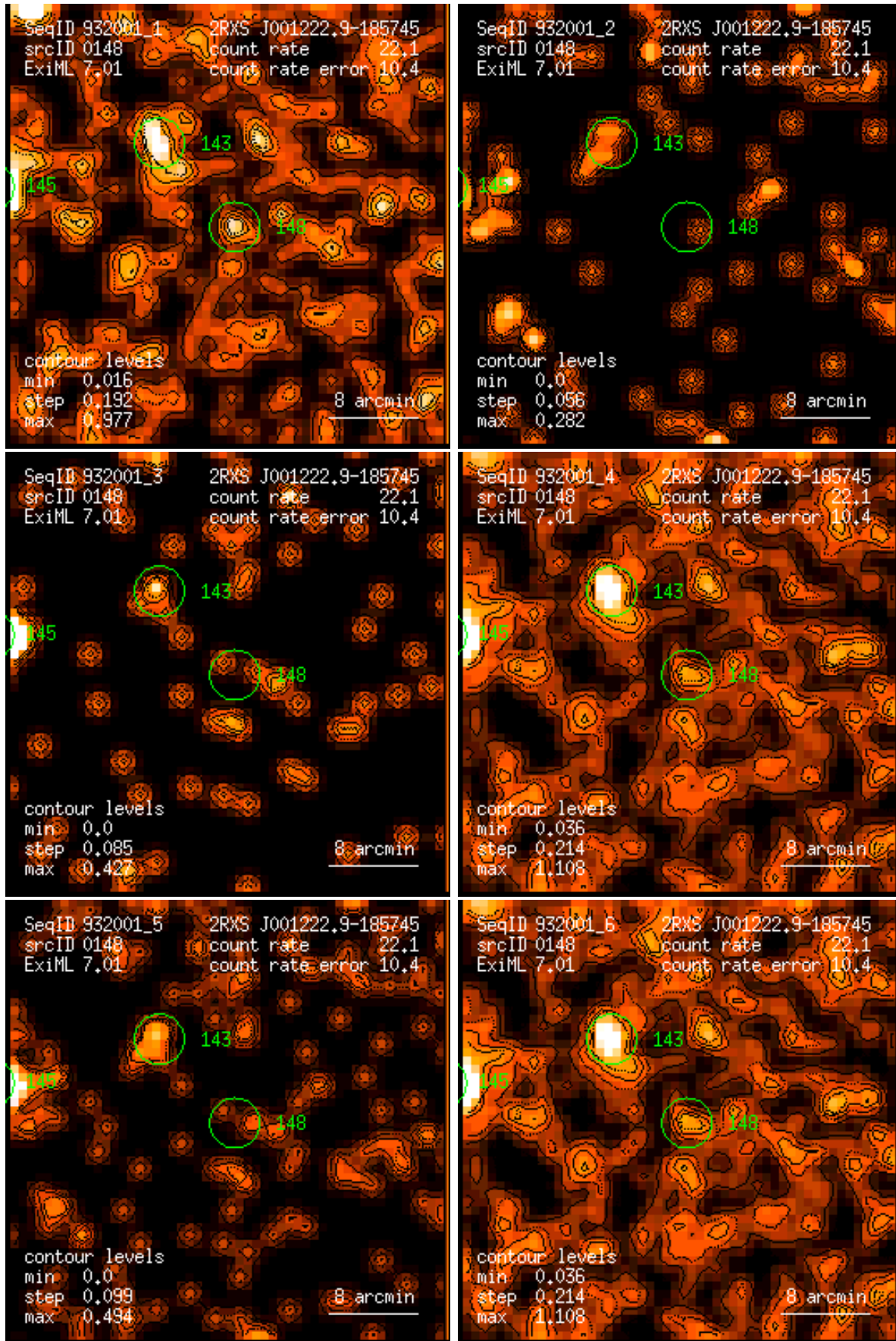
Figure 148: RASS 932001: detection 0148: band rate images, Gaussian filter: (1) PSPC channels 11 – 41, (2) 52 – 90, (3) 91 – 201, (4) 11 – 235, (5) 52 – 201, (6) 11 – 201. Broad band rates in counts/ks. Band rate contour levels in counts/ks/arcmin 2 .
