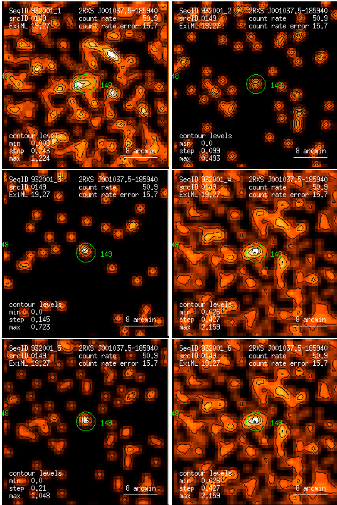
Figure 149: RASS 932001: detection 0149: band rate images, Gaussian filter: (1) PSPC channels 11 – 41, (2) 52 – 90, (3) 91 – 201, (4) 11 – 235, (5) 52 – 201, (6) 11 – 201. Broad band rates in counts/ks. Band rate contour levels in counts/ks/arcmin 2 .
