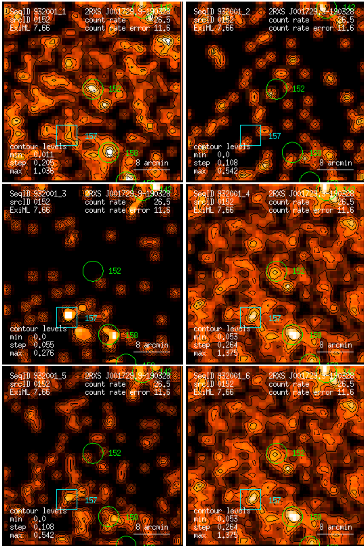
Figure 152: RASS 932001: detection 0152: band rate images, Gaussian filter: (1) PSPC channels 11 – 41, (2) 52 – 90, (3) 91 – 201, (4) 11 – 235, (5) 52 – 201, (6) 11 – 201. Broad band rates in counts/ks. Band rate contour levels in counts/ks/arcmin 2 .
