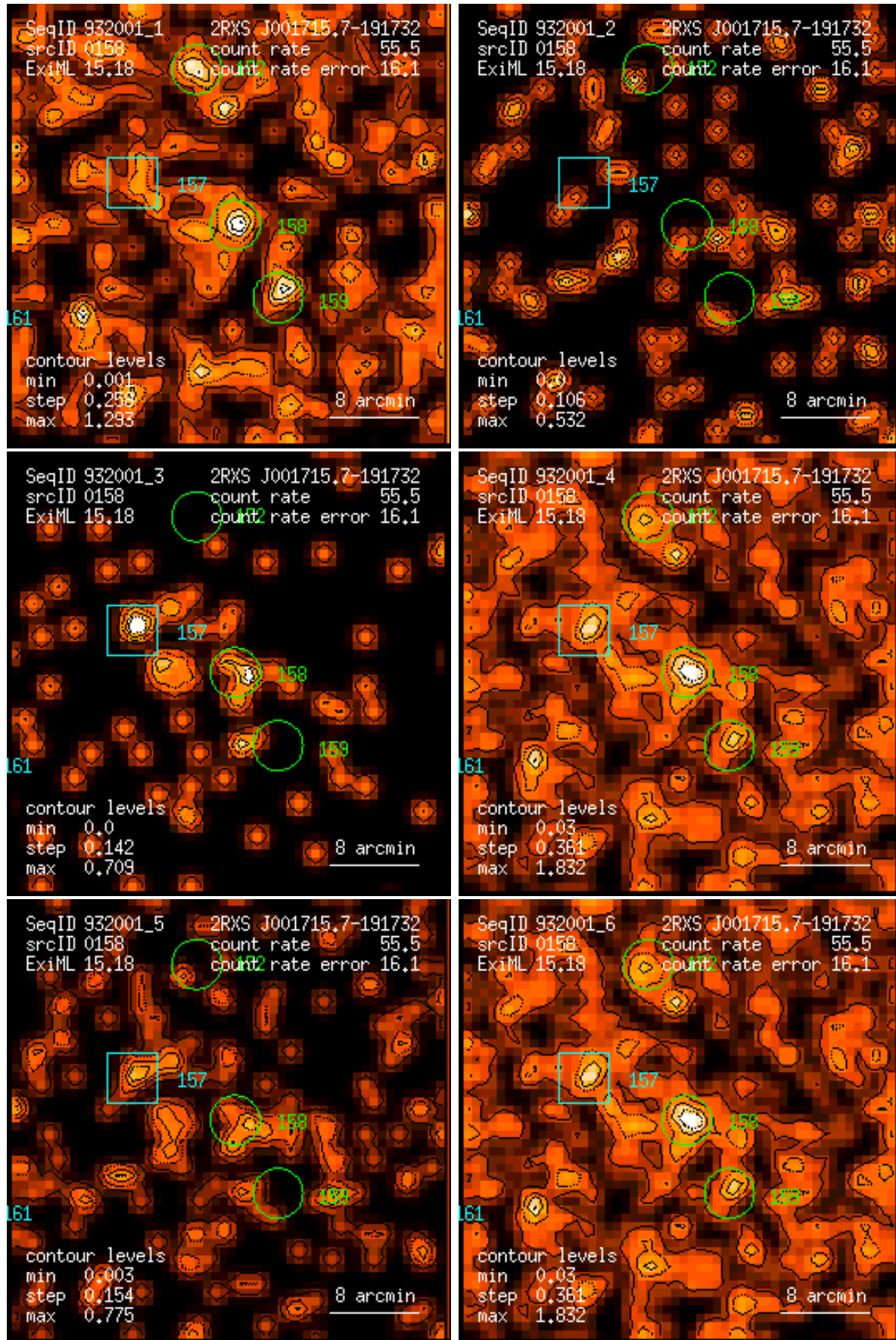
Figure 158: RASS 932001: detection 0158: band rate images, Gaussian filter: (1) PSPC channels 11 – 41, (2) 52 – 90, (3) 91 – 201, (4) 11 – 235, (5) 52 – 201, (6) 11 – 201. Broad band rates in counts/ks. Band rate contour levels in counts/ks/arcmin 2 .
