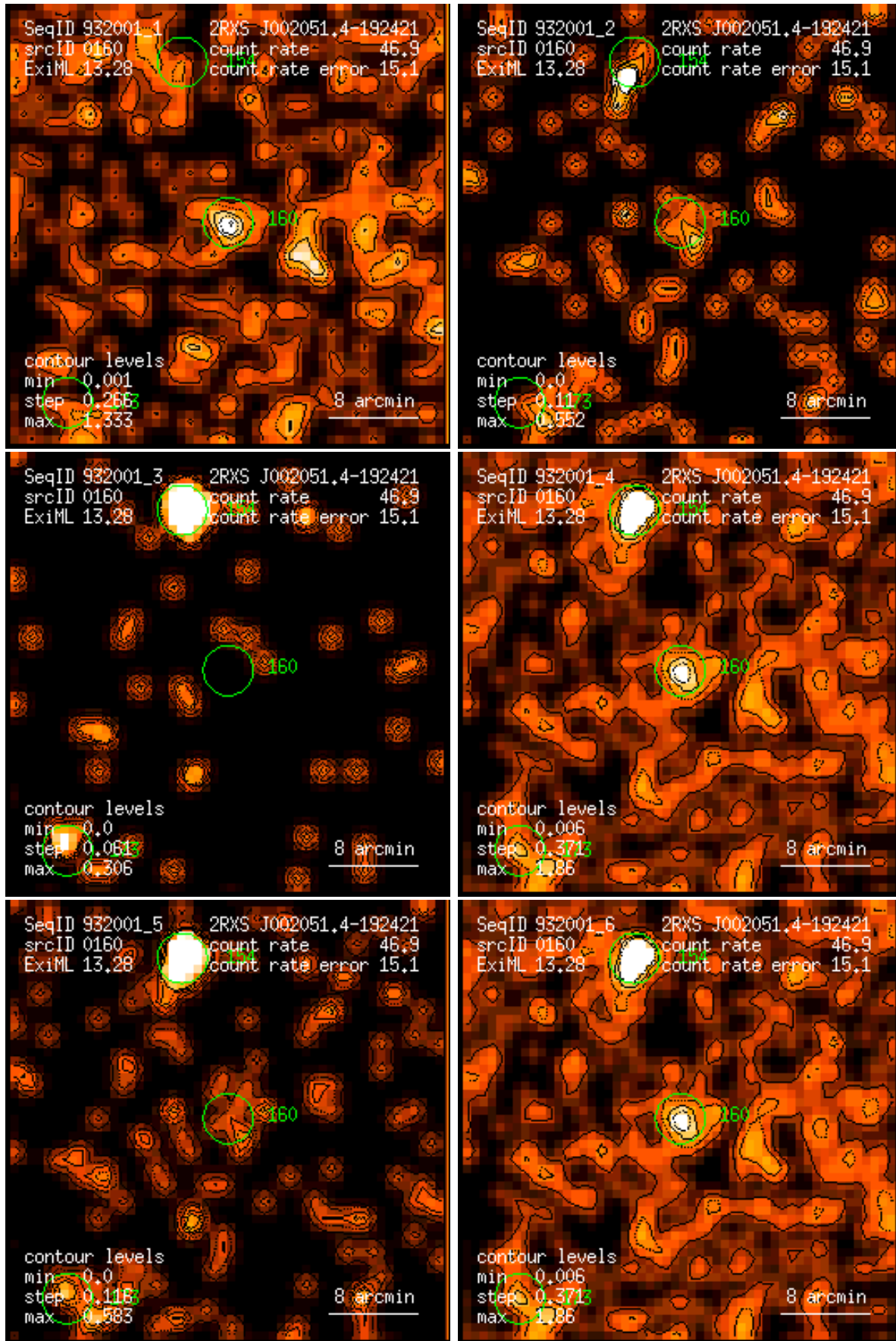
Figure 160: RASS 932001: detection 0160: band rate images, Gaussian filter: (1) PSPC channels 11 – 41, (2) 52 – 90, (3) 91 – 201, (4) 11 – 235, (5) 52 – 201, (6) 11 – 201. Broad band rates in counts/ks. Band rate contour levels in counts/ks/arcmin 2 .
