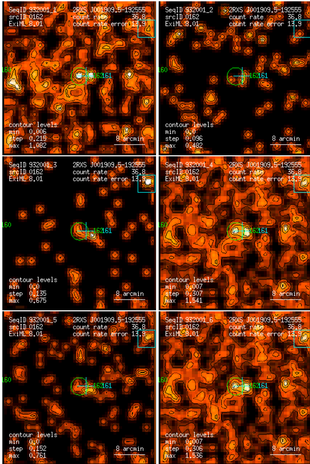
Figure 162: RASS 932001: detection 0162: band rate images, Gaussian filter: (1) PSPC channels 11 – 41, (2) 52 – 90, (3) 91 – 201, (4) 11 – 235, (5) 52 – 201, (6) 11 – 201. Broad band rates in counts/ks. Band rate contour levels in counts/ks/arcmin 2 .
