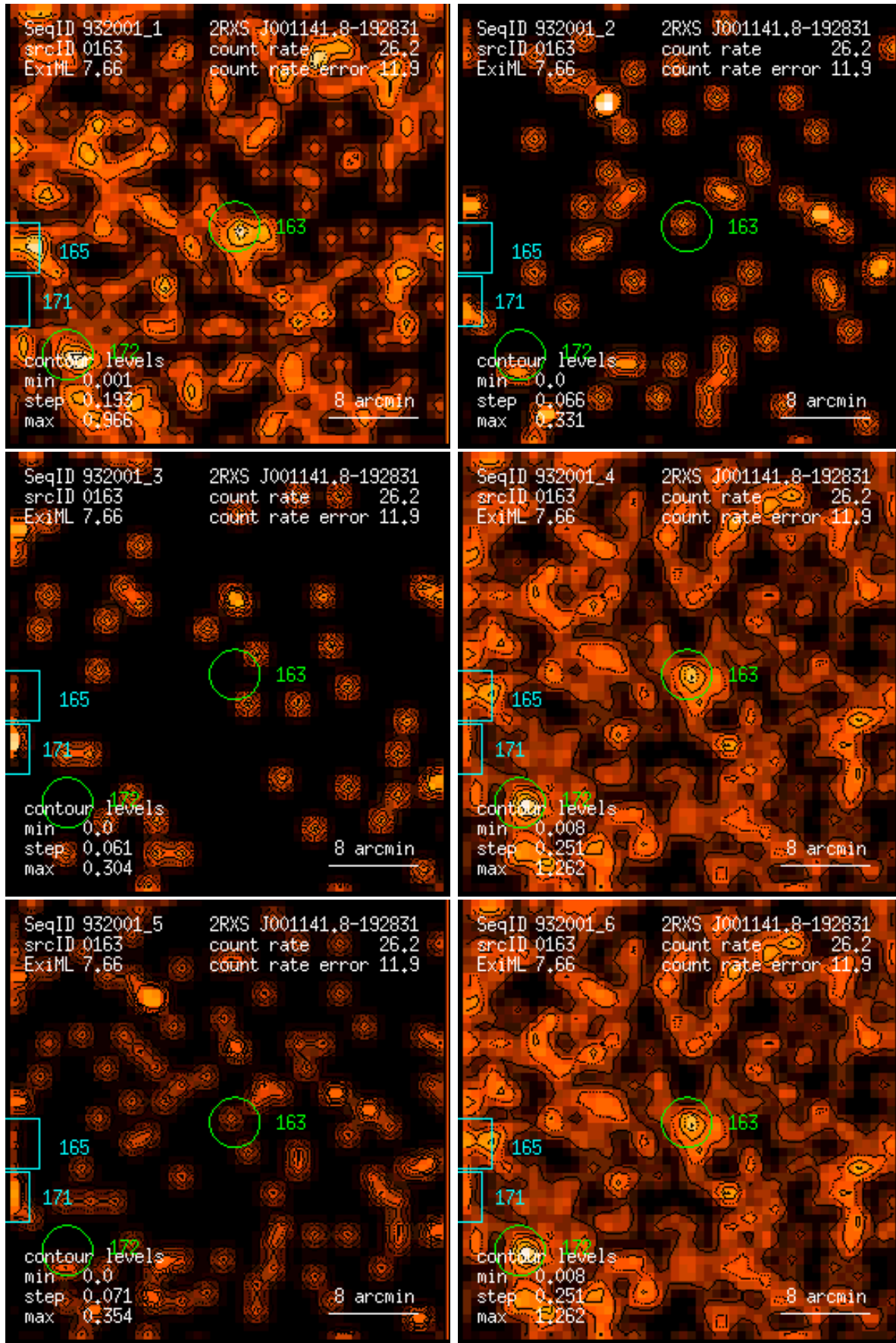
Figure 163: RASS 932001: detection 0163: band rate images, Gaussian filter: (1) PSPC channels 11 – 41, (2) 52 – 90, (3) 91 – 201, (4) 11 – 235, (5) 52 – 201, (6) 11 – 201. Broad band rates in counts/ks. Band rate contour levels in counts/ks/arcmin 2 .
