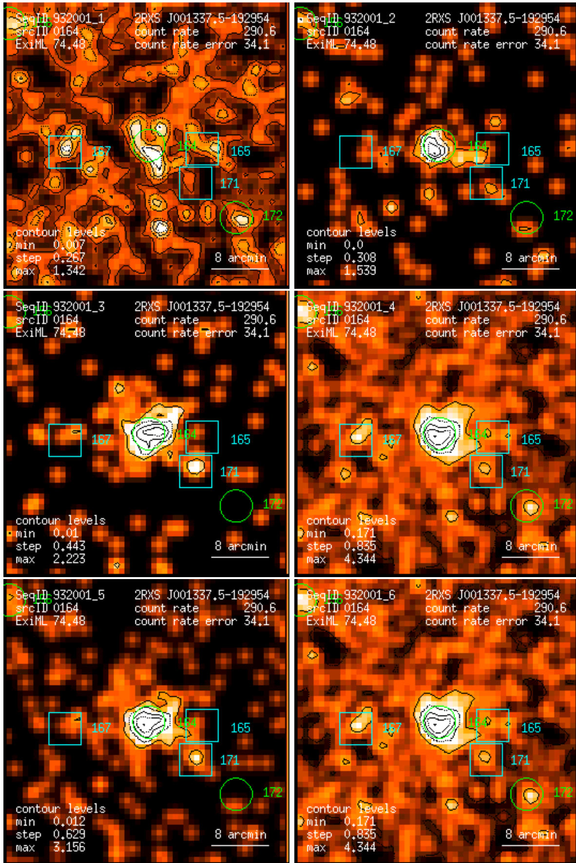
Figure 164: RASS 932001: detection 0164: band rate images, Gaussian filter: (1) PSPC channels 11 – 41, (2) 52 – 90, (3) 91 – 201, (4) 11 – 235, (5) 52 – 201, (6) 11 – 201. Broad band rates in counts/ks. Band rate contour levels in counts/ks/arcmin 2 .
