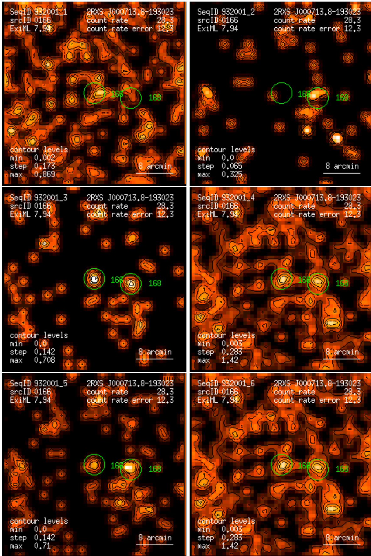
Figure 166: RASS 932001: detection 0166: band rate images, Gaussian filter: (1) PSPC channels 11 – 41, (2) 52 – 90, (3) 91 – 201, (4) 11 – 235, (5) 52 – 201, (6) 11 – 201. Broad band rates in counts/ks. Band rate contour levels in counts/ks/arcmin 2 .
