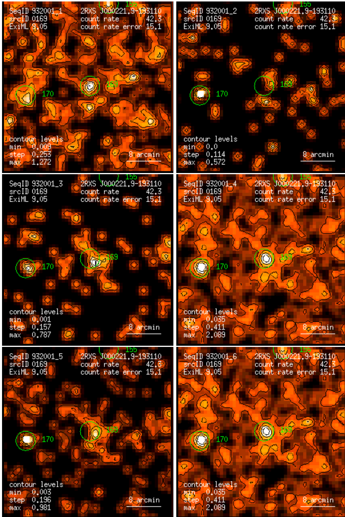
Figure 169: RASS 932001: detection 0169: band rate images, Gaussian filter: (1) PSPC channels 11 – 41, (2) 52 – 90, (3) 91 – 201, (4) 11 – 235, (5) 52 – 201, (6) 11 – 201. Broad band rates in counts/ks. Band rate contour levels in counts/ks/arcmin 2 .
